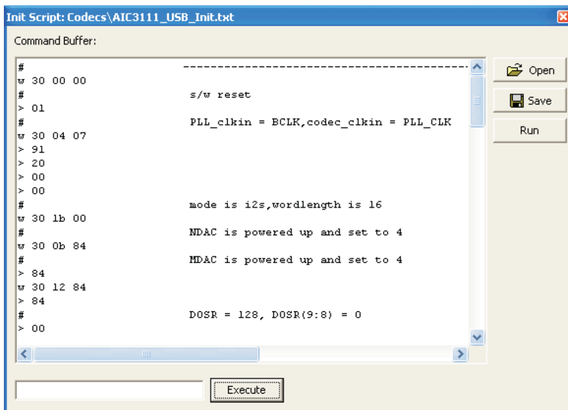
Figure 2. Initialization Script
